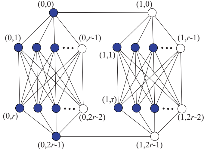
Figure 4.4: The double jewel, J_{2,r}
