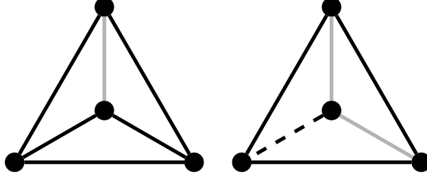
Figure 2: Representative elements of \mathcal{H}(2, 1, 0) and \mathcal{H}(0, 2, 1) .
