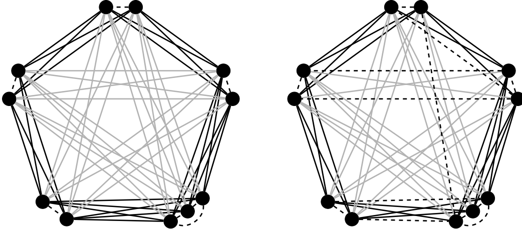
Figure 1: G_{ex}(11) and another element of \mathcal{G}_{11}
